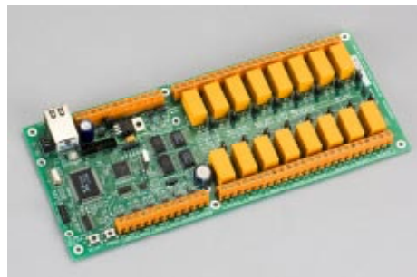
16 Digital Output IO Board for BioScan
